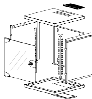
EXPLODED VIEW
