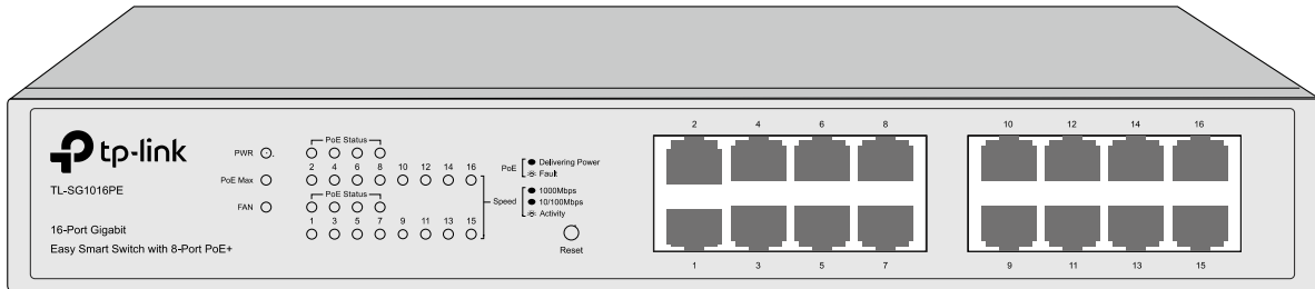
Figure 2-6 Front Panel of TL-SG1016PE
