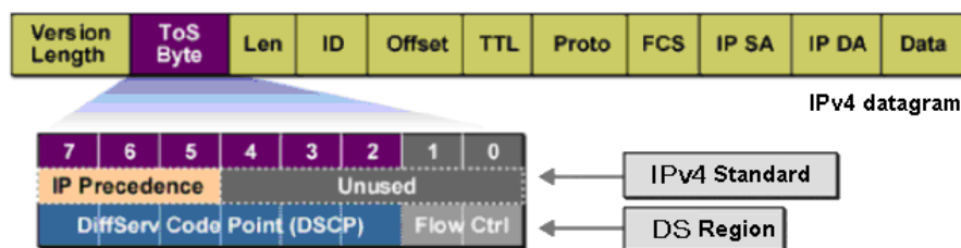
Figure 8-4 IP datagram
