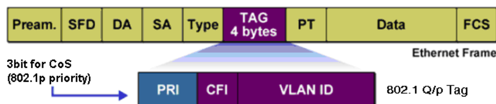
Figure 8-2 802.1Q frame
