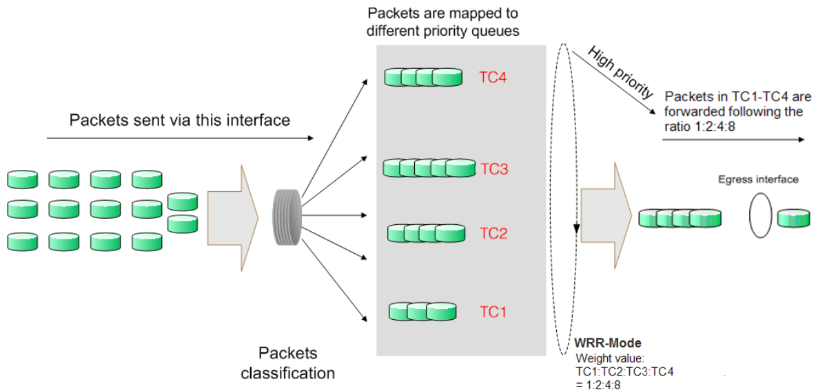
Figure 8-1 QoS function
