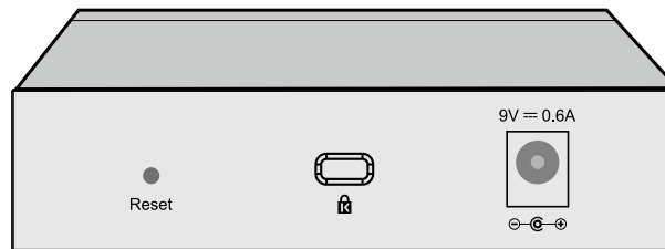
Figure 2-7 Rear Panel of TL-SG105E
