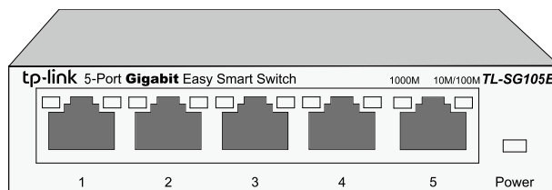
Figure 2-1 Front Panel of TL-SG105E
