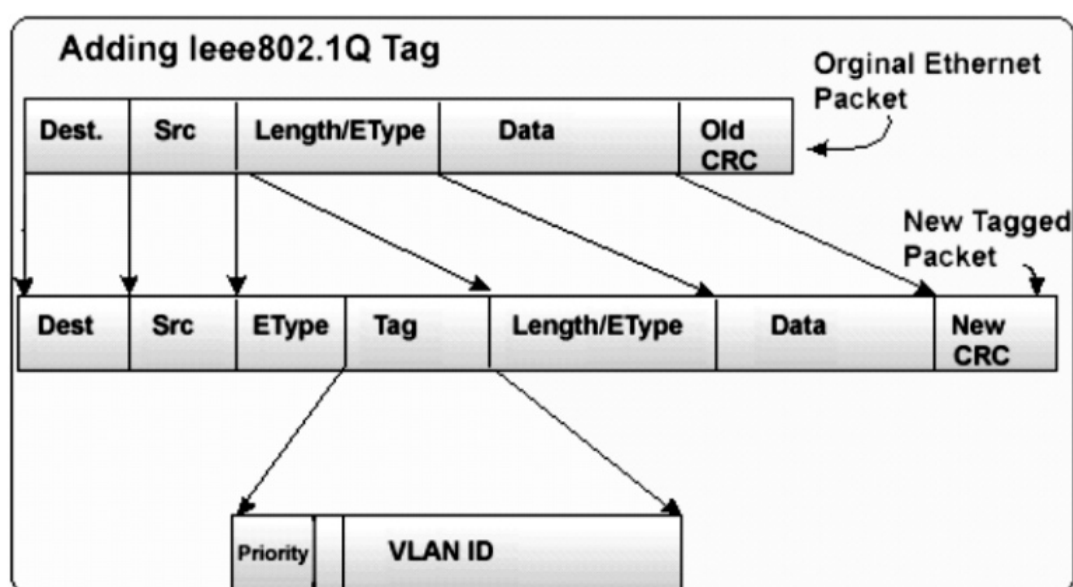
Figure 7-2 IEEE 802.1Q frame
