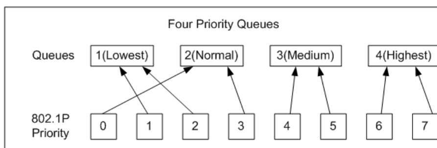
Figure 8-3 Map 802.1P priority
