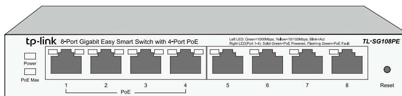
Figure 2-3 Front Panel of TL-SG108PE
