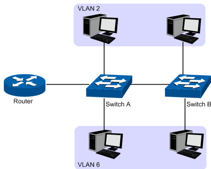
Figure 7-1 VLAN implementation
