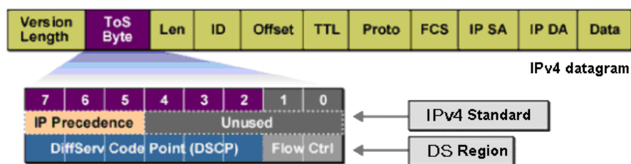
Figure 7-3 IP datagram
