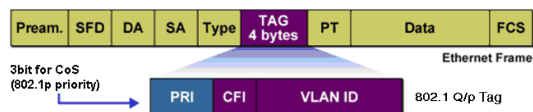
Figure 7-2 802.1Q Frame
