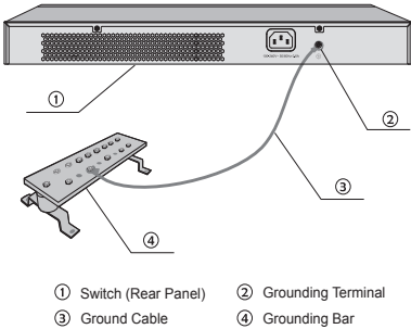
Figure 3-1 Connecting to the Grounding Bar
