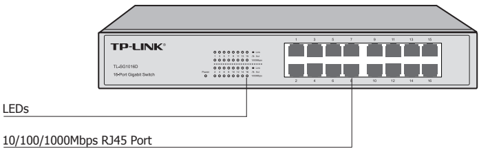
Figure 1-5 Front Panel of TL-SG1016D
