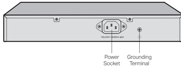
Figure 1-14 Rear Panel of TL-SG1008PE
