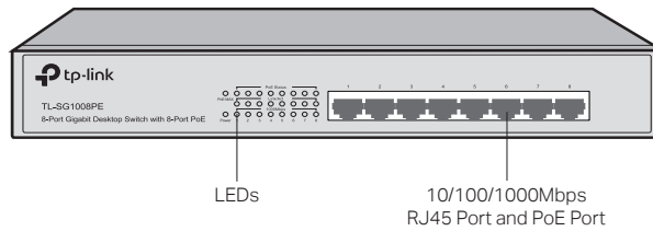
Figure 1-7 Front Panel of TL-SG1008PE
