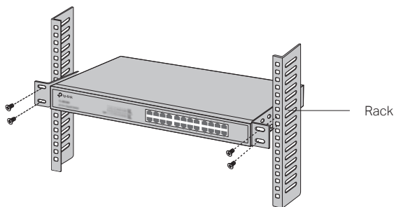
Figure 2-3 Rack Installation
